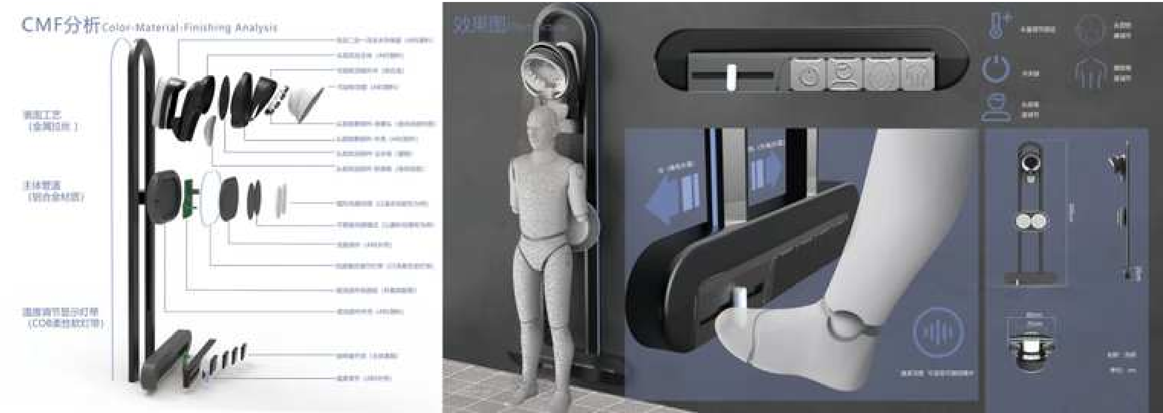
Modules, controls and human-scale relationships
