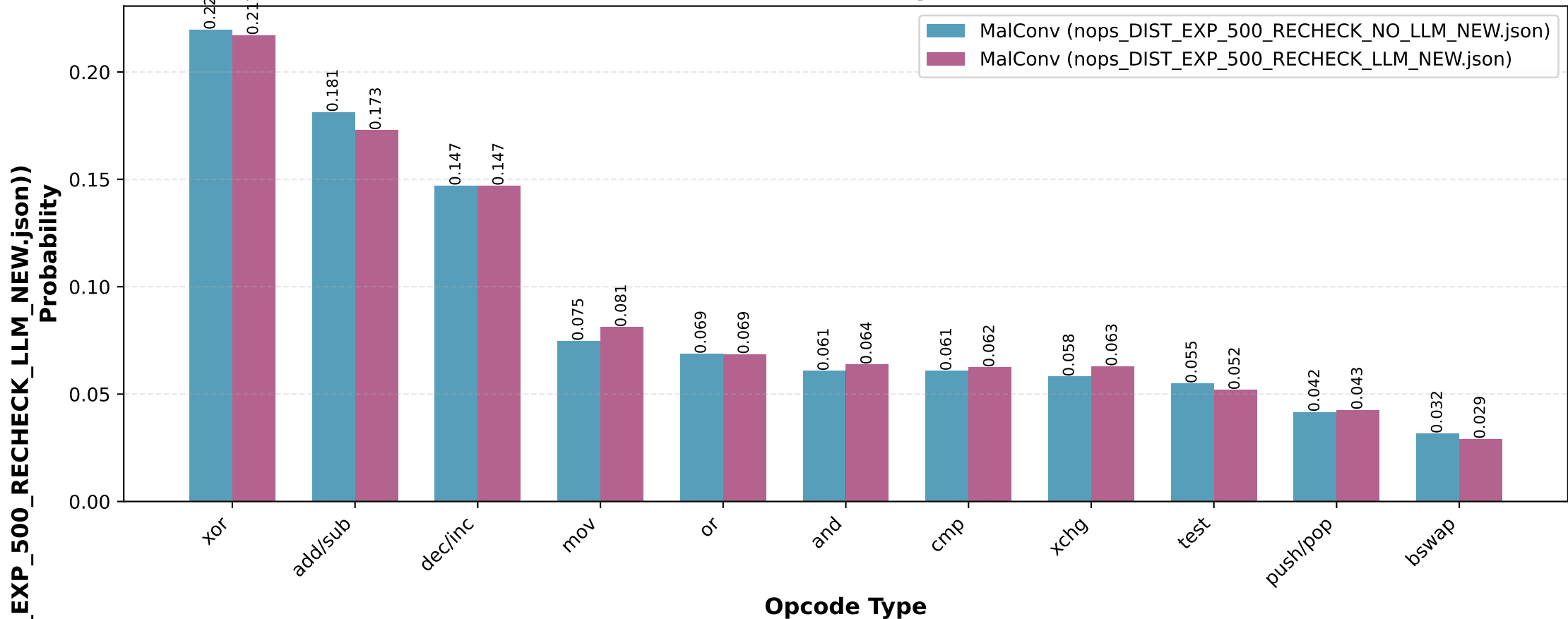
Distribution Comparison
