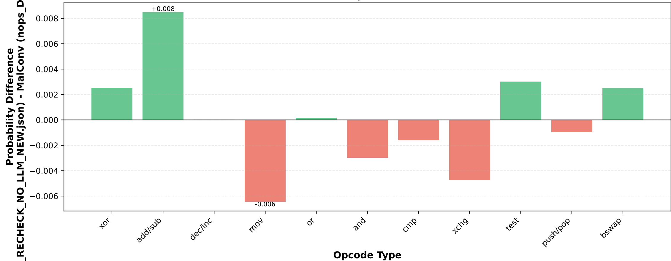
Probability Differences
