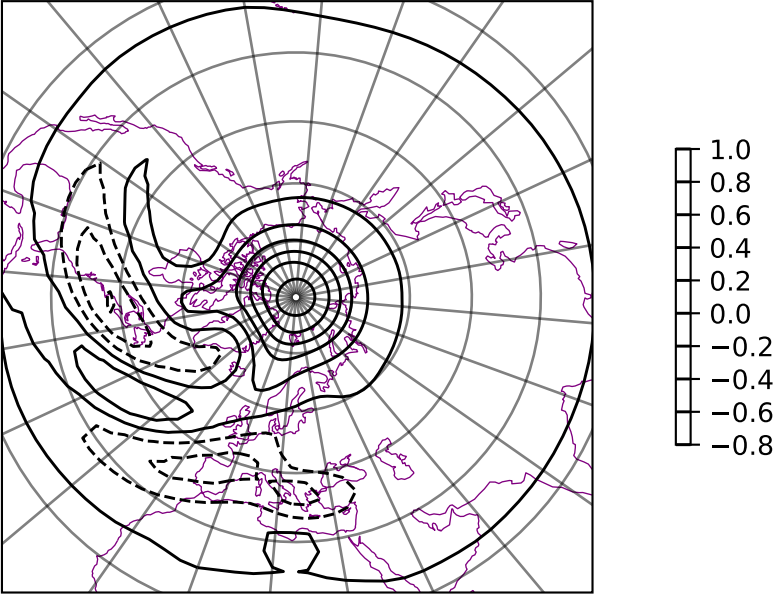
SQG u diff 200 hpa 0240h - T031 expid=101
