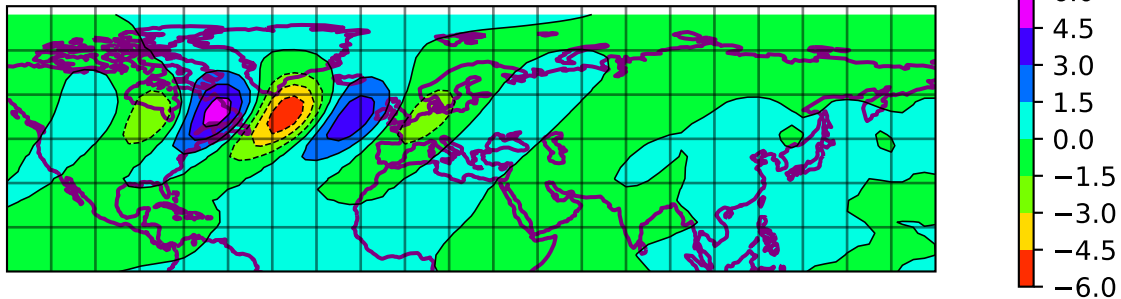
SQG v 200 hpa 0240h - T031 expid=104
