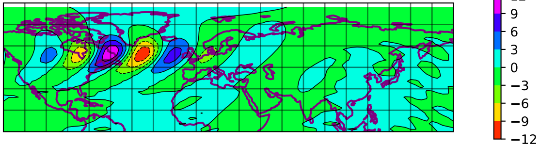
SQG v 500 hpa 0240h - T031 expid=104
