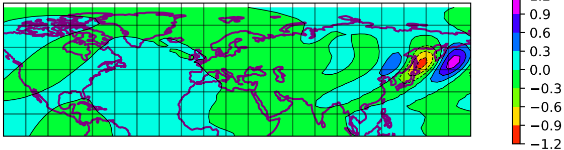
SQG v 800 hpa 0120h - T031 expid=104
