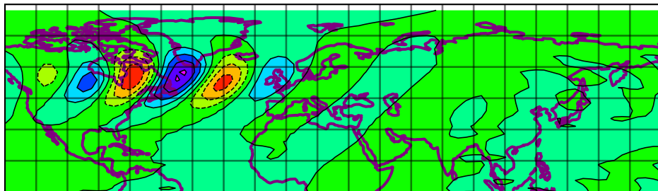
SQG v 800 hpa 0240h - T031 expid=104
