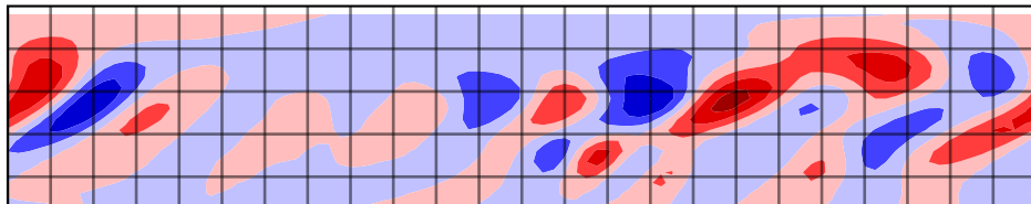
SQG v diff2 800 hpa 0360h - T031 expid=104
