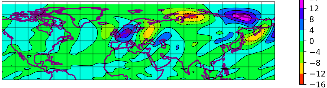
SQG v 800 hpa 0360h - T031 expid=104
