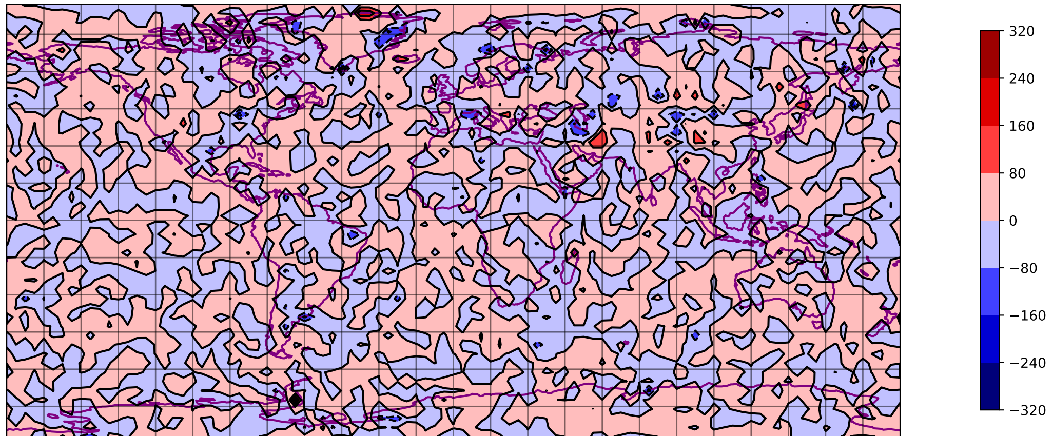
SQG DIV @ 1000 hpa 00 h - T031 ERA5
