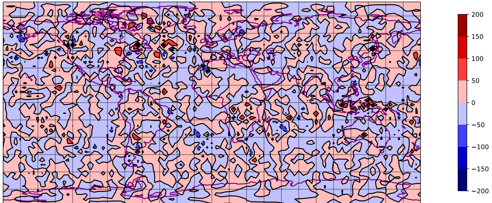
SQG DIV @ 200 hpa 00 h - T031 ERA5
