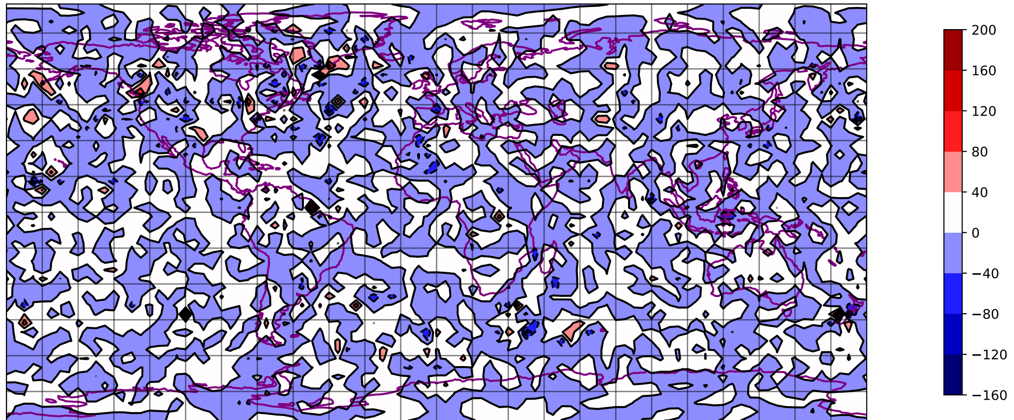
SQG DIV @ 350 hpa 00 h - T031 ERA5
