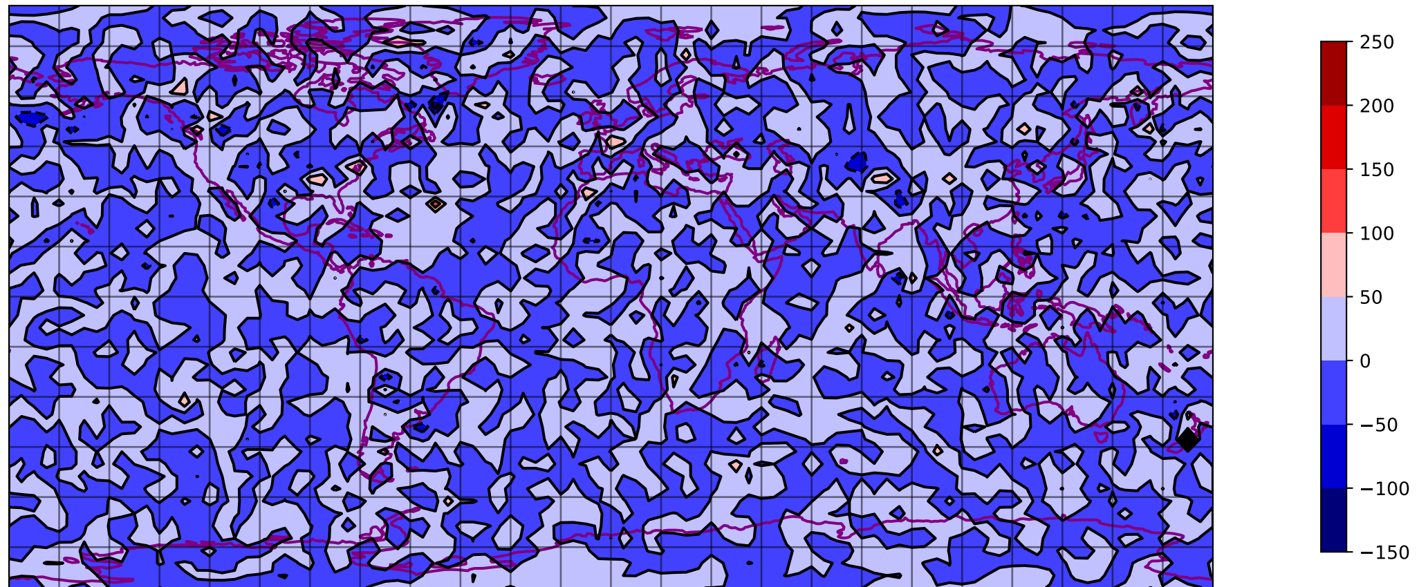
SQG DIV @ 500 hpa 00 h - T031 ERA5
