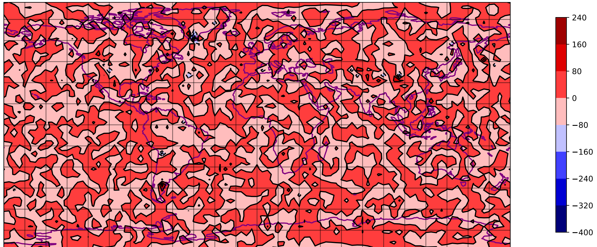
SQG DIV @ 650 hpa 00 h - T031 ERA5
