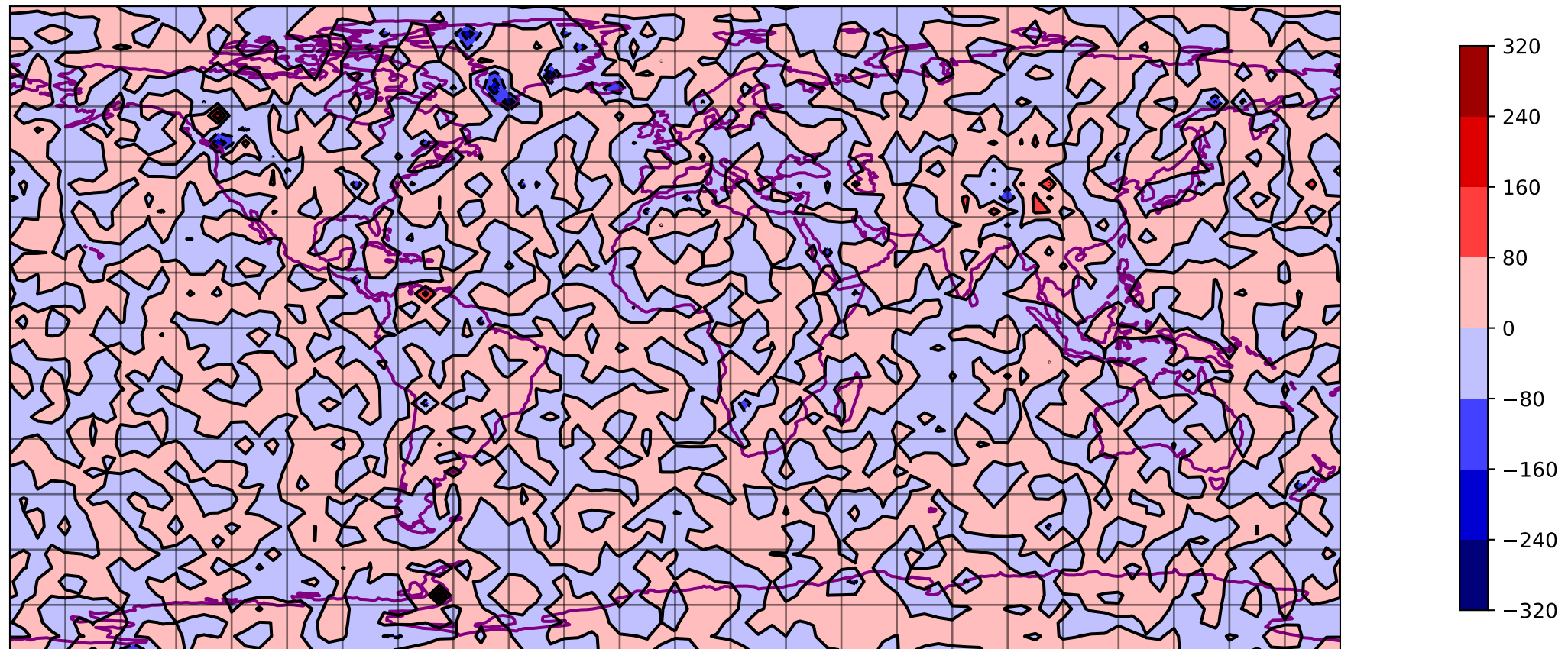
SQG DIV @ 800 hpa 00 h - T031 ERA5
