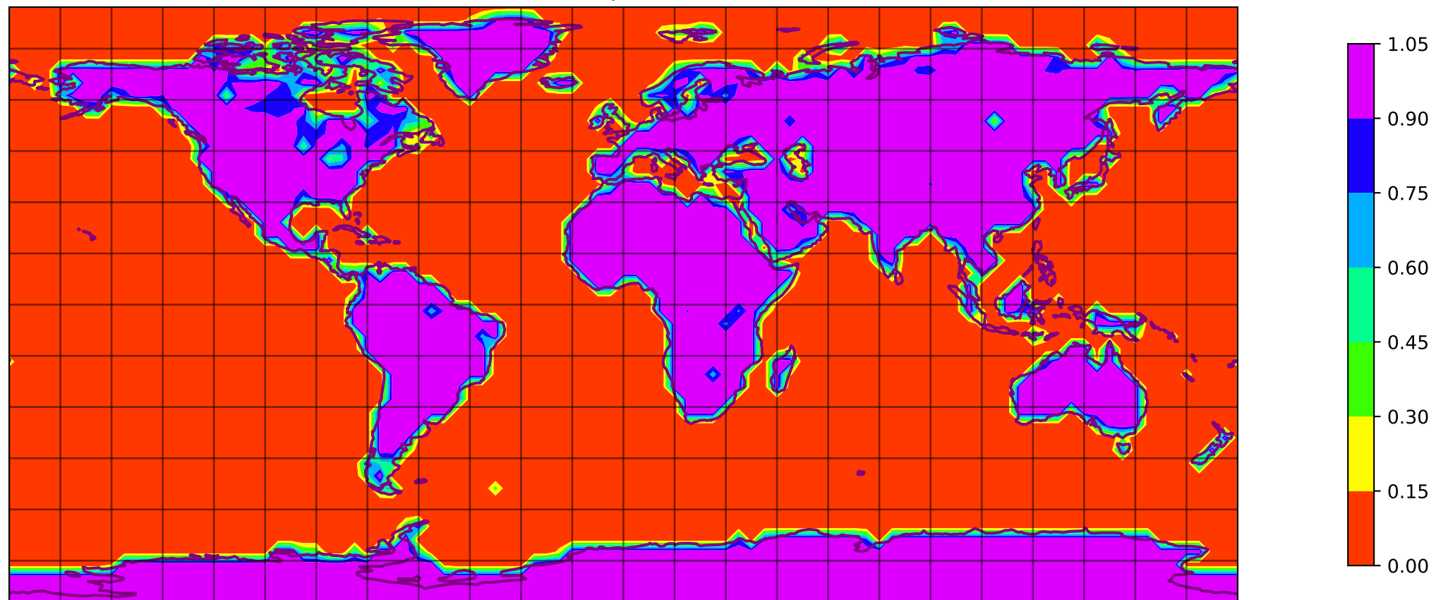
SQG LSM @ 200 hpa 00 h - T031 ERA5
