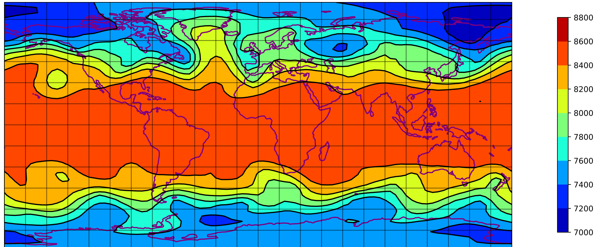
SQG PHI @ 350 hpa 00 h - T031 ERA5
