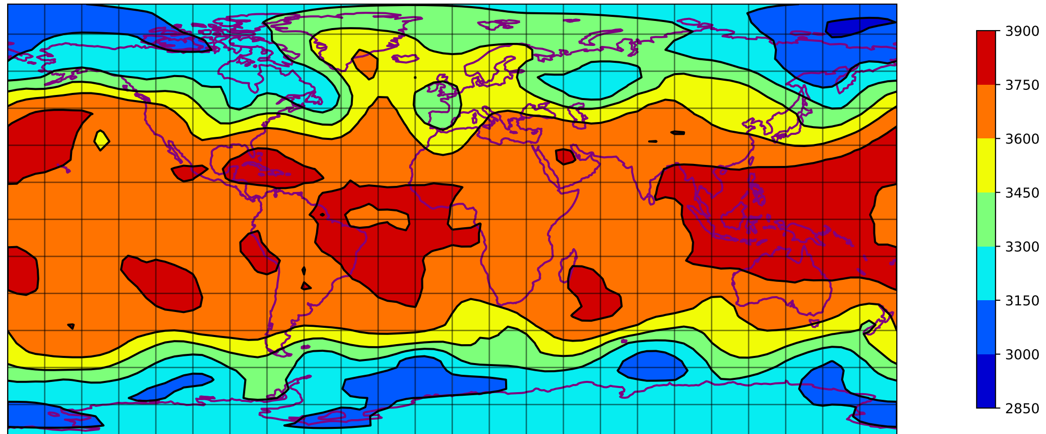
SQG PHI @ 650 hpa 00 h - T031 ERA5
