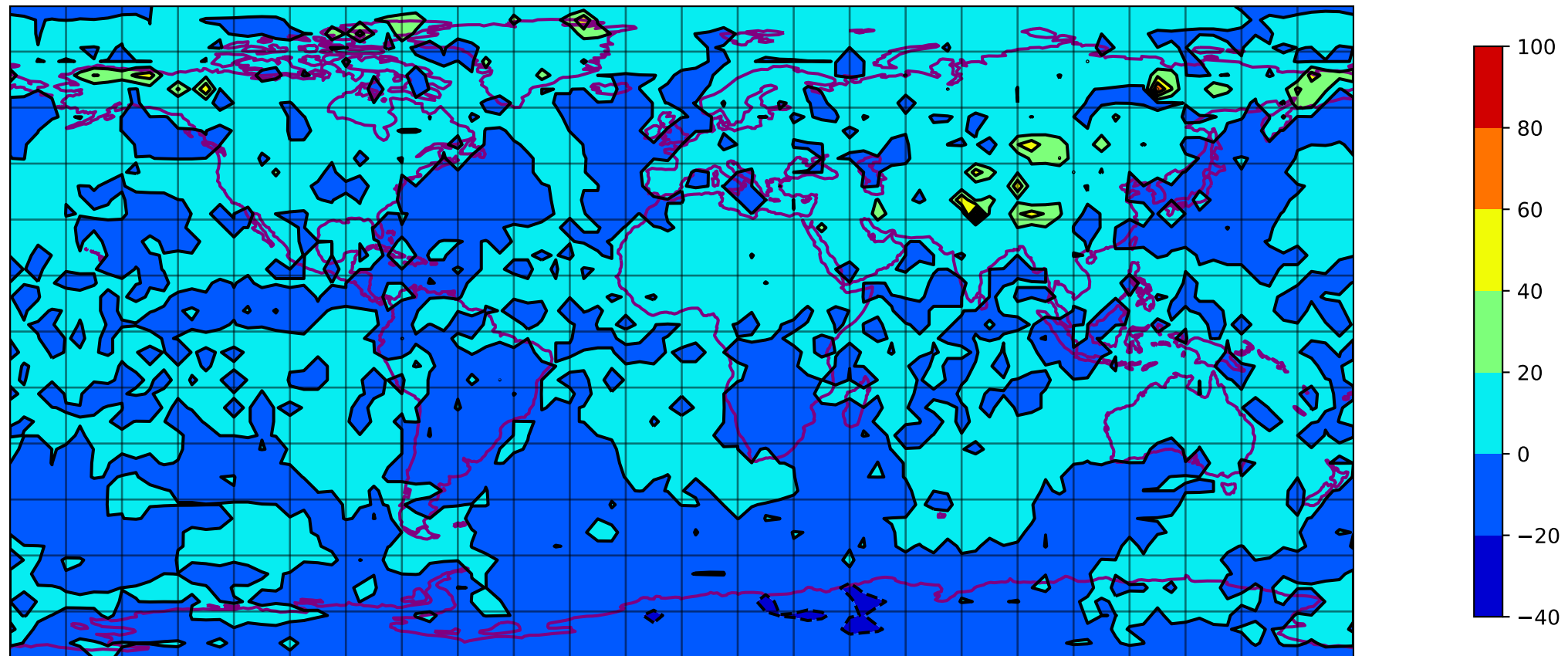
SQG PV @ 1000 hpa 00 h - T031 ERA5
