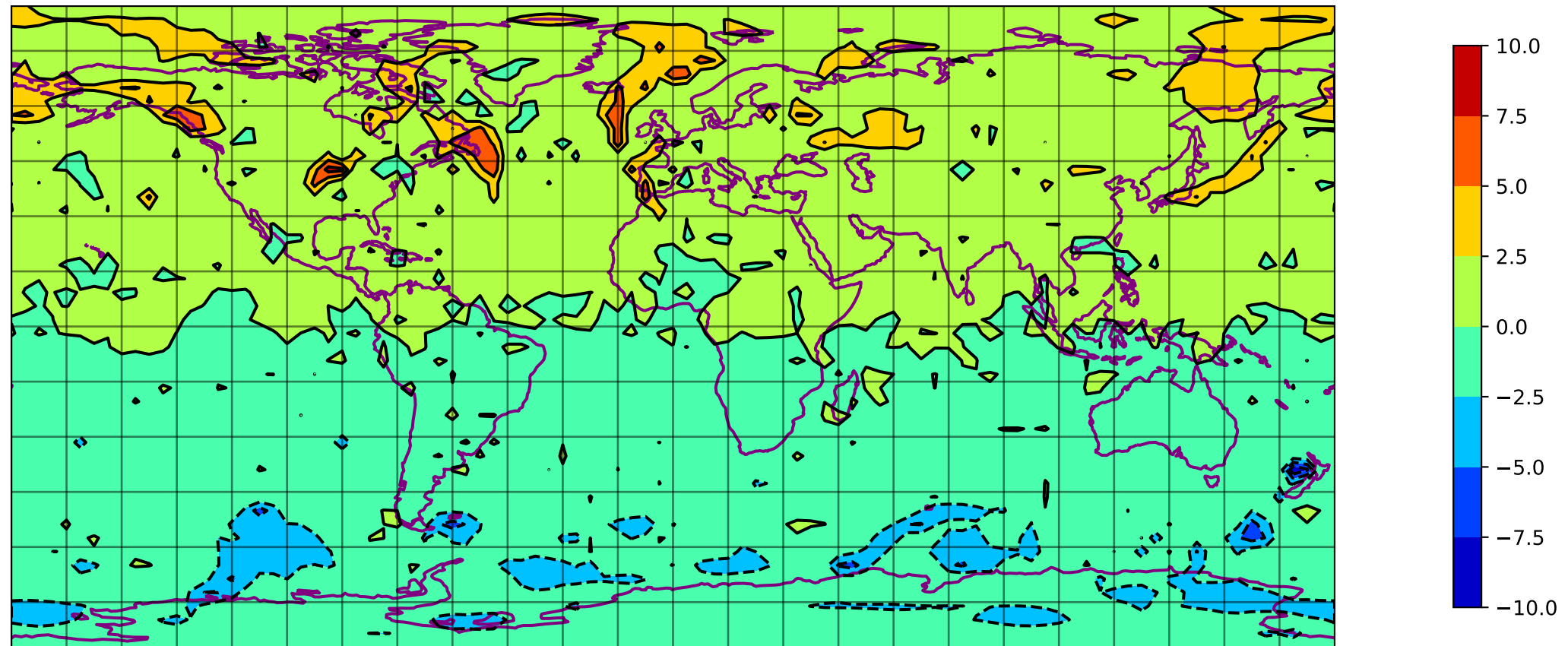
SQG PV @ 350 hpa 00 h - T031 ERA5
