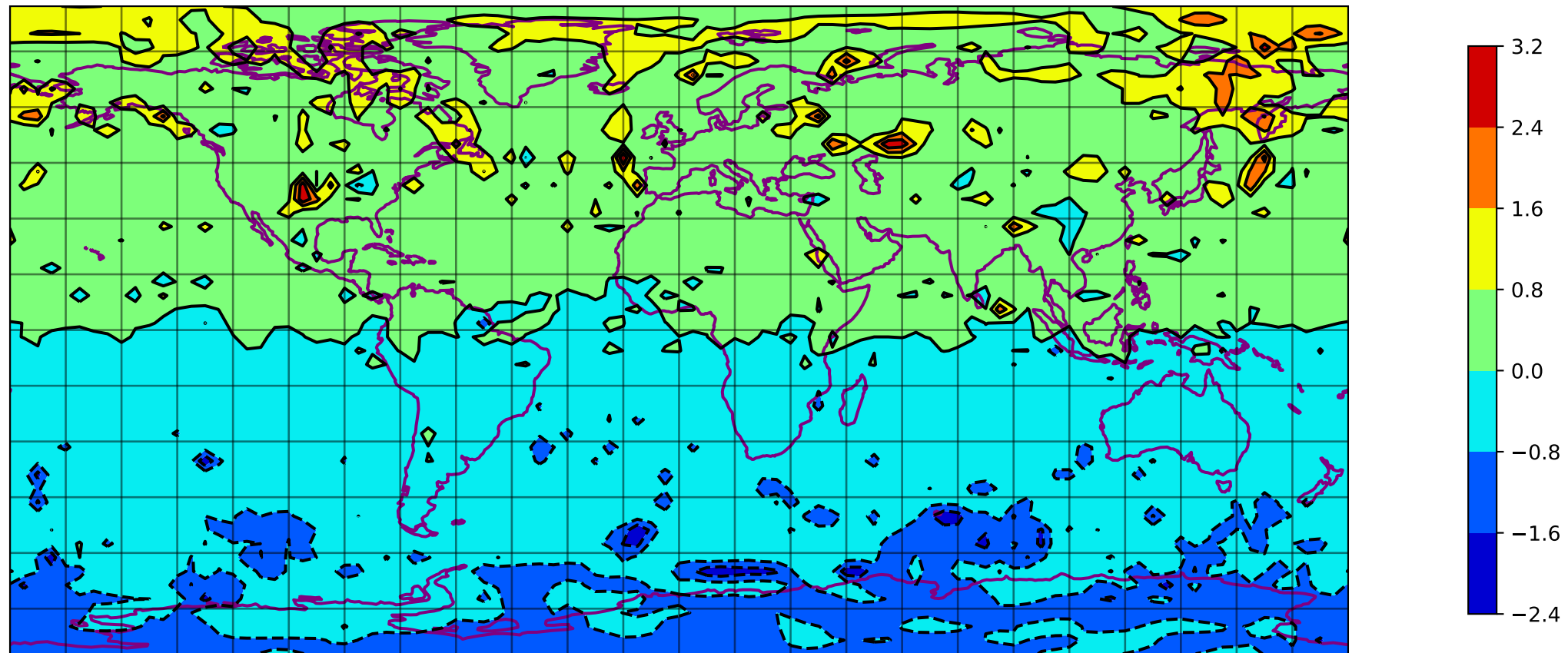
SQG PV @ 500 hpa 00 h - T031 ERA5
