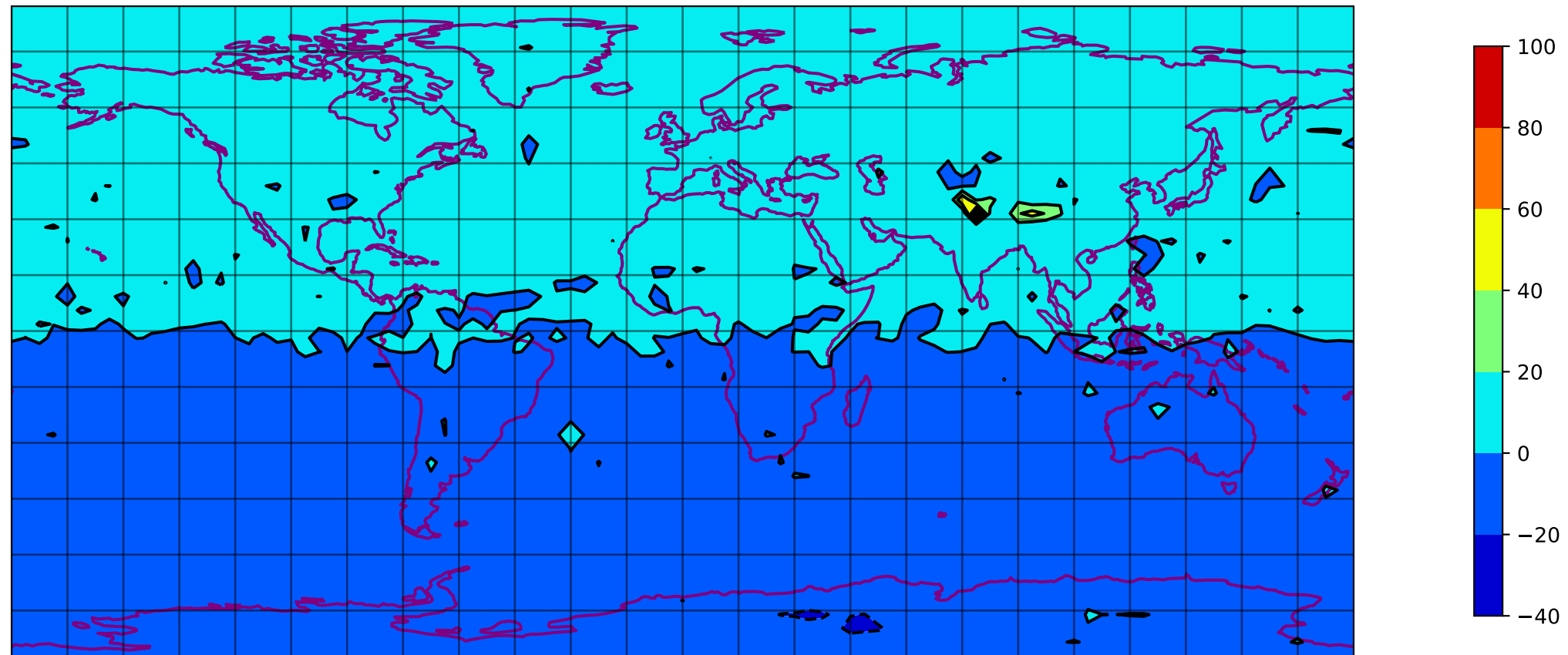
SQG PV @ 650 hpa 00 h - T031 ERA5
