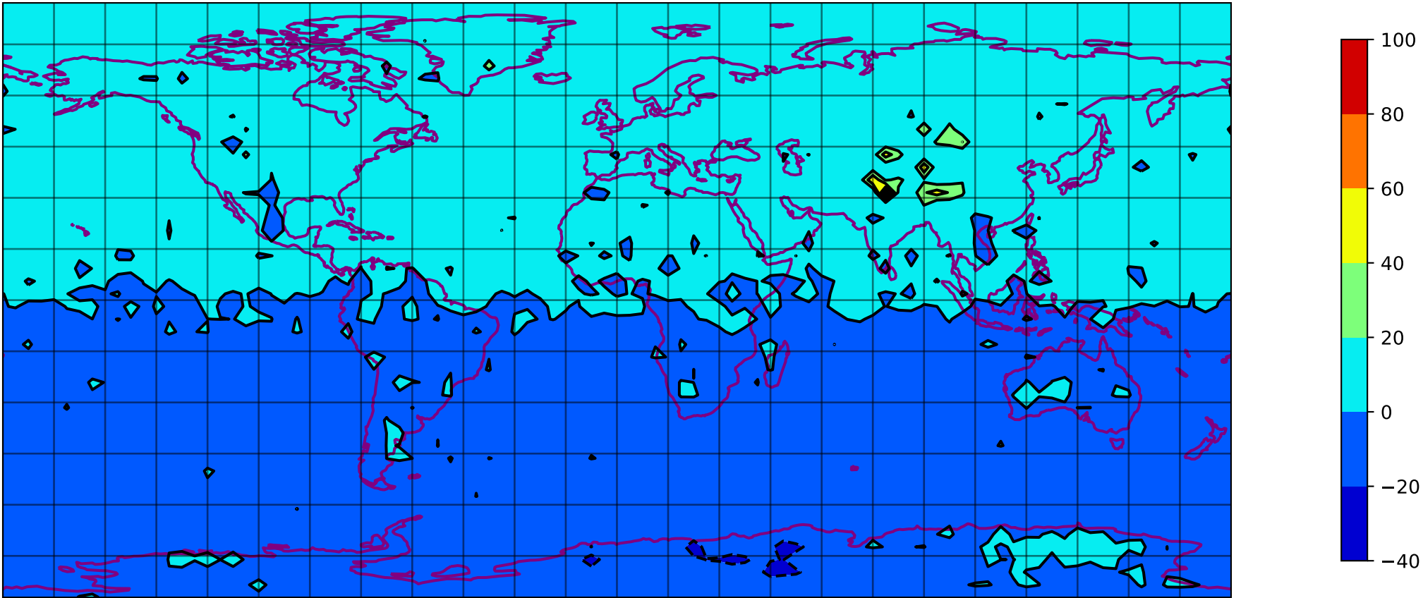
SQG PV @ 800 hpa 00 h - T031 ERA5
