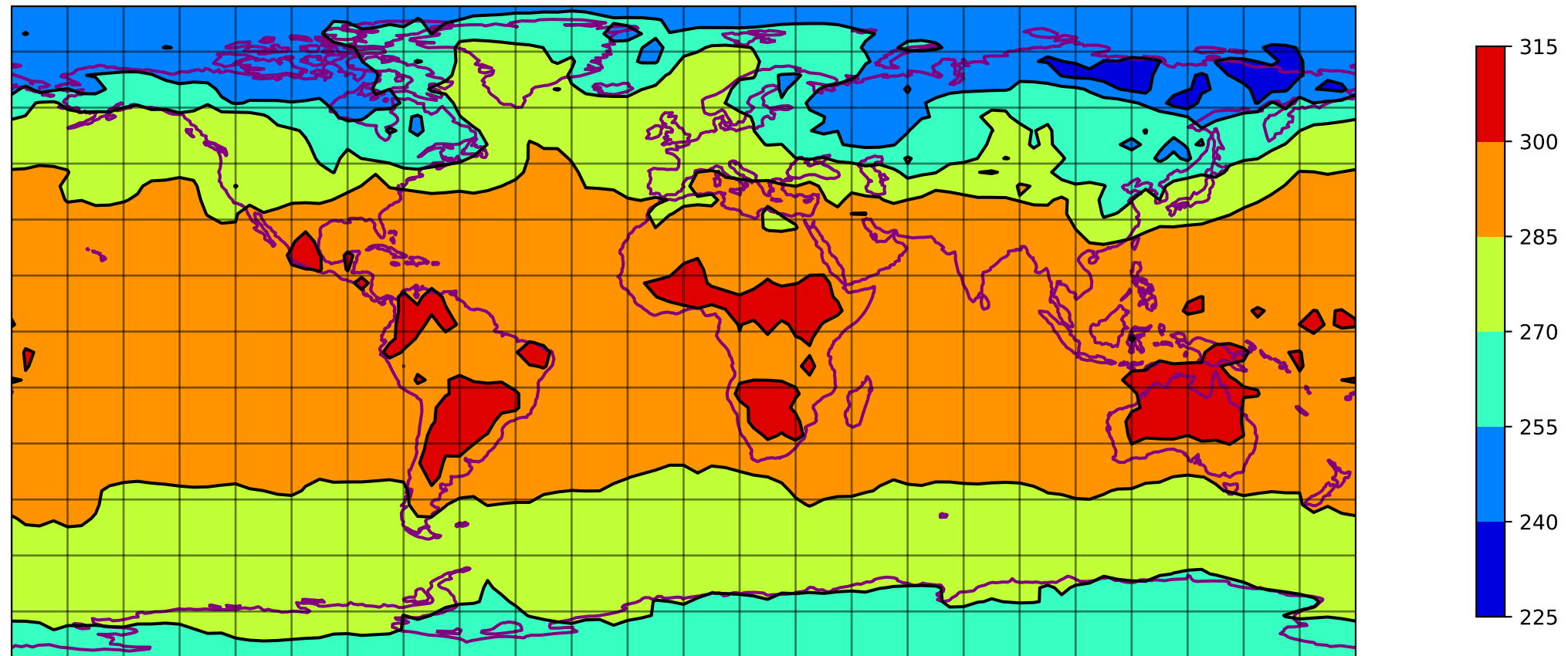
SQG T @ 1000 hpa 00 h - T031 ERA5
