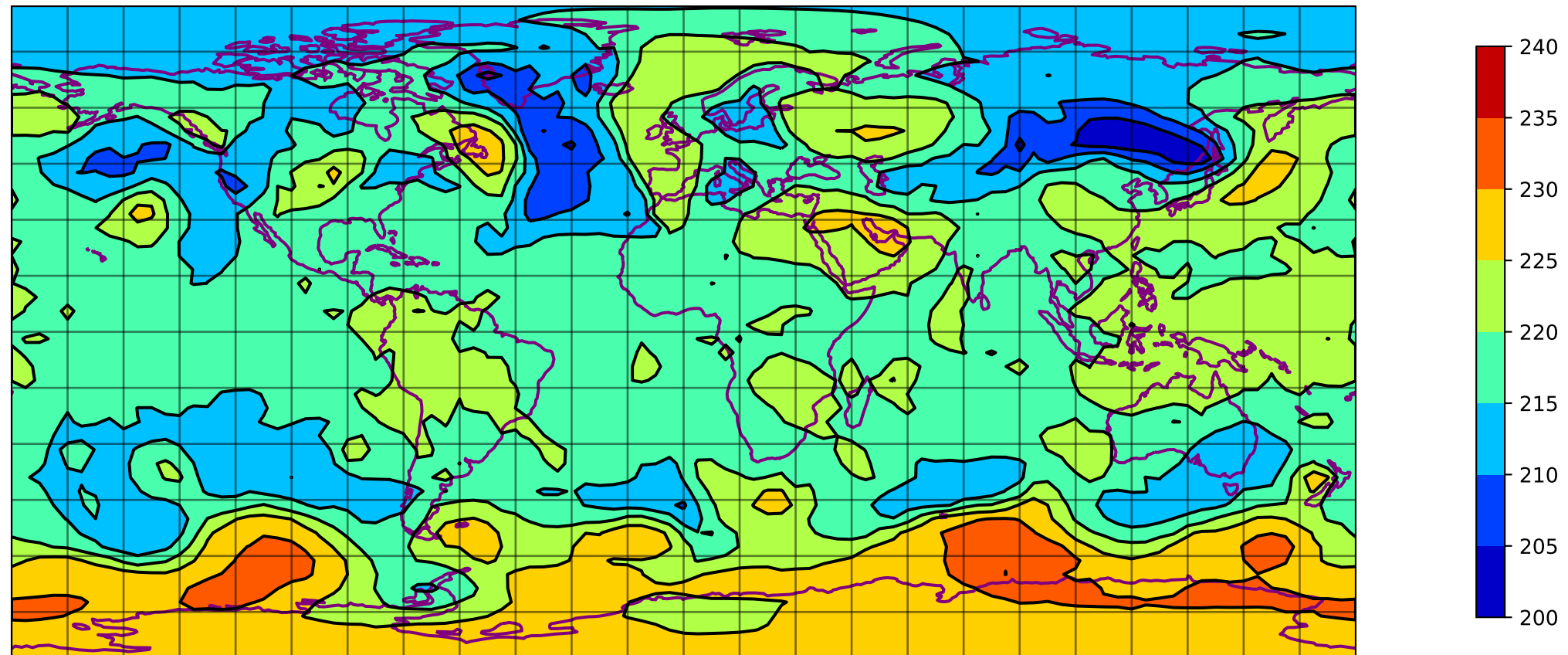
SQG T @ 200 hpa 00 h - T031 ERA5
