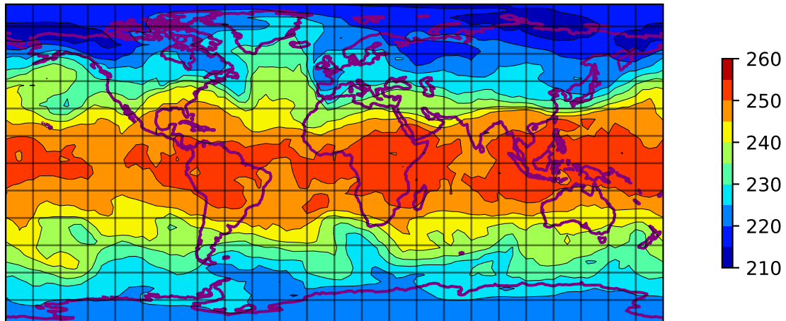
SQG T @ 350 hpa 00 h - T031 ERA5
