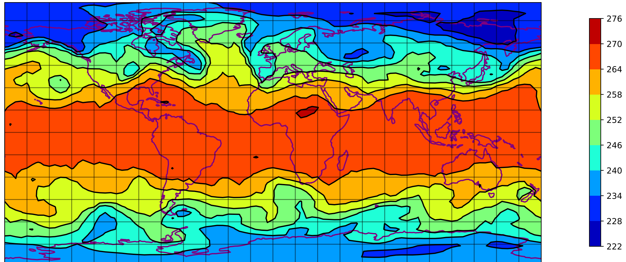
SQG T @ 500 hpa 00 h - T031 ERA5
