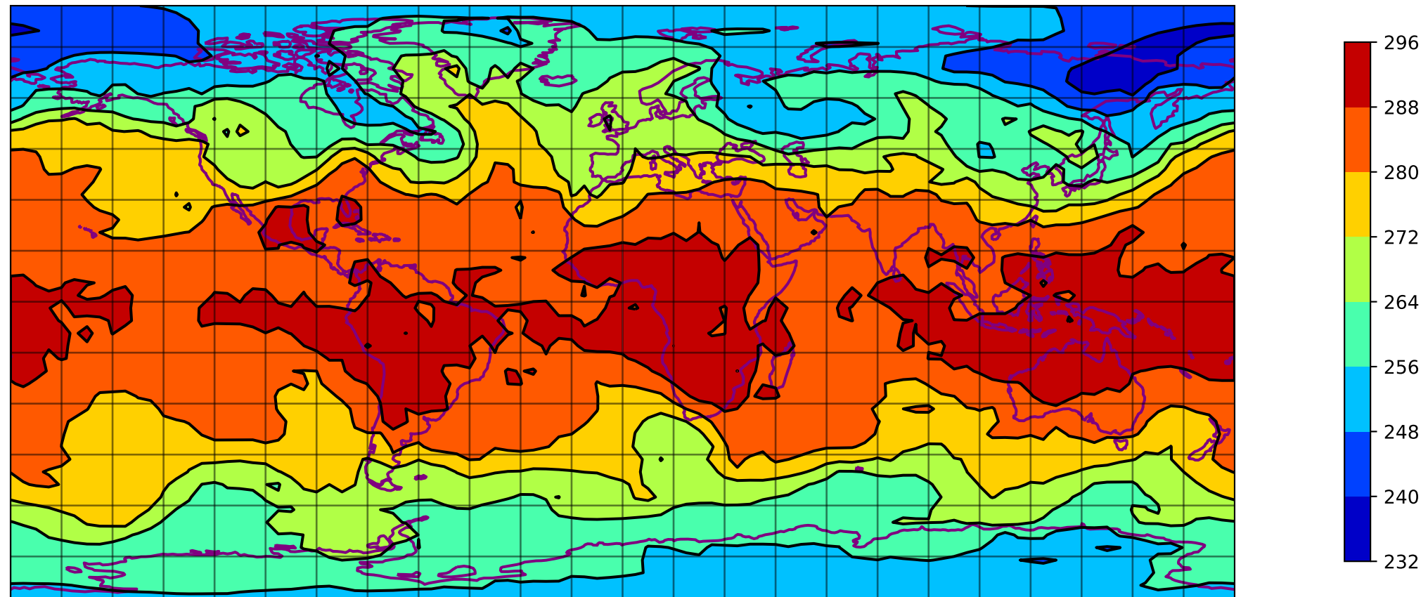
SQG T @ 800 hpa 00 h - T031 ERA5
