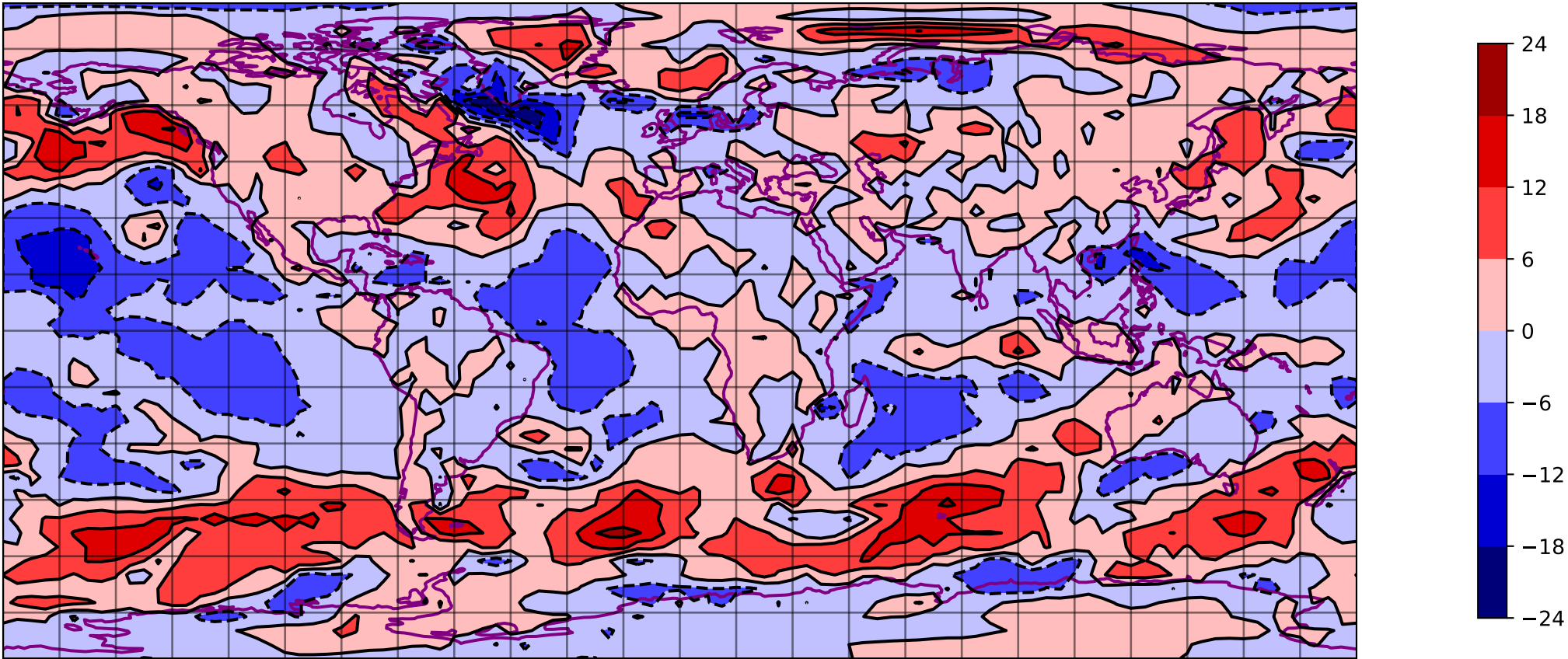
SQG U @ 1000 hpa 00 h - T031 ERA5
