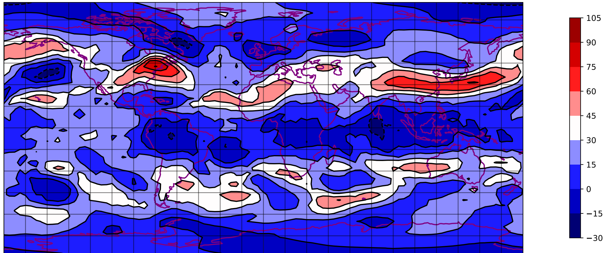
SQG U @ 200 hpa 00 h - T031 ERA5
