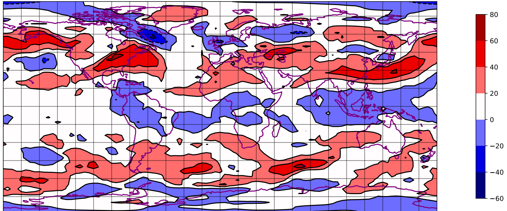
SQG U @ 350 hpa 00 h - T031 ERA5
