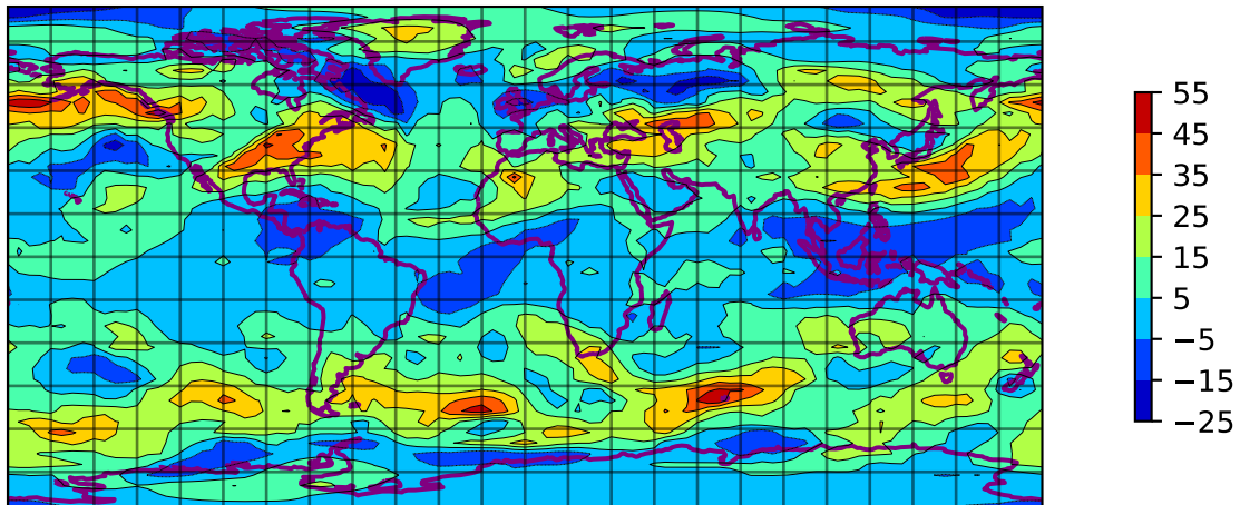
SQG U @ 500 hpa 00 h - T031 ERA5
