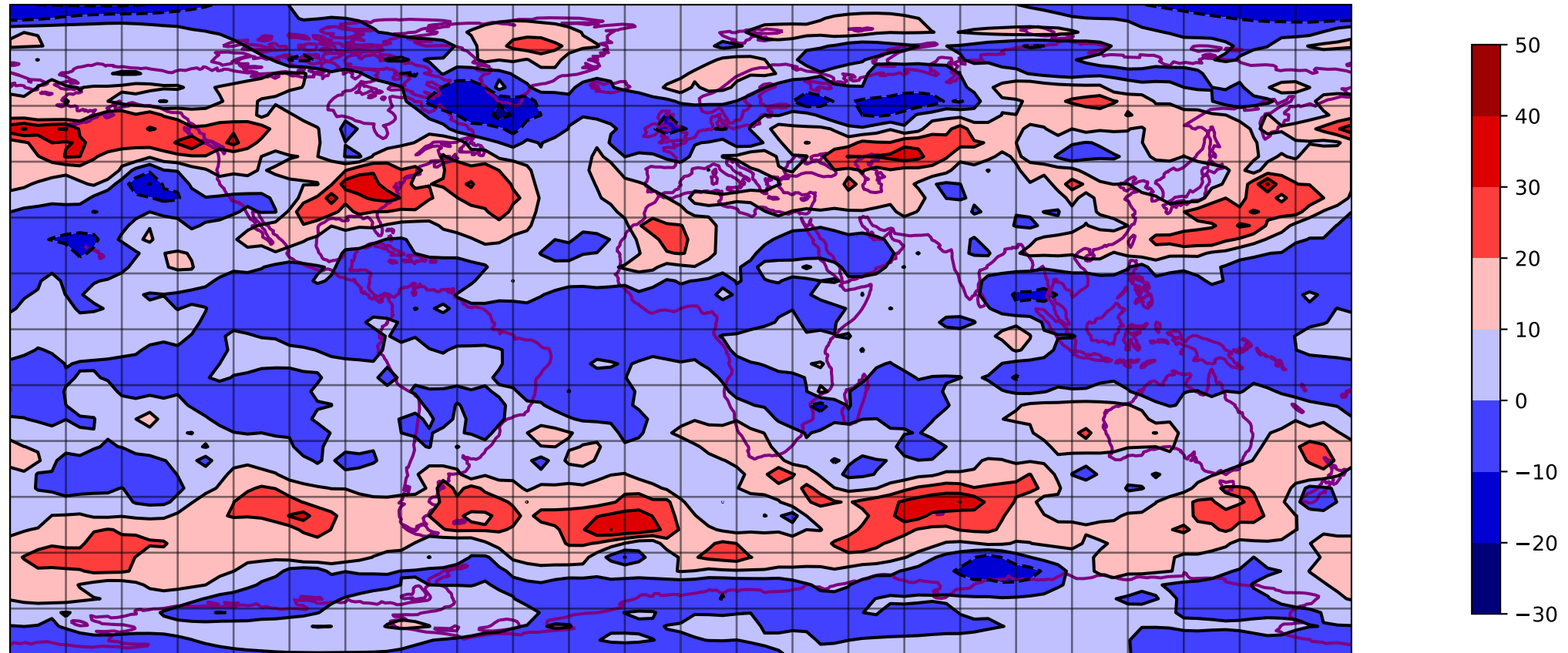
SQG U @ 650 hpa 00 h - T031 ERA5
