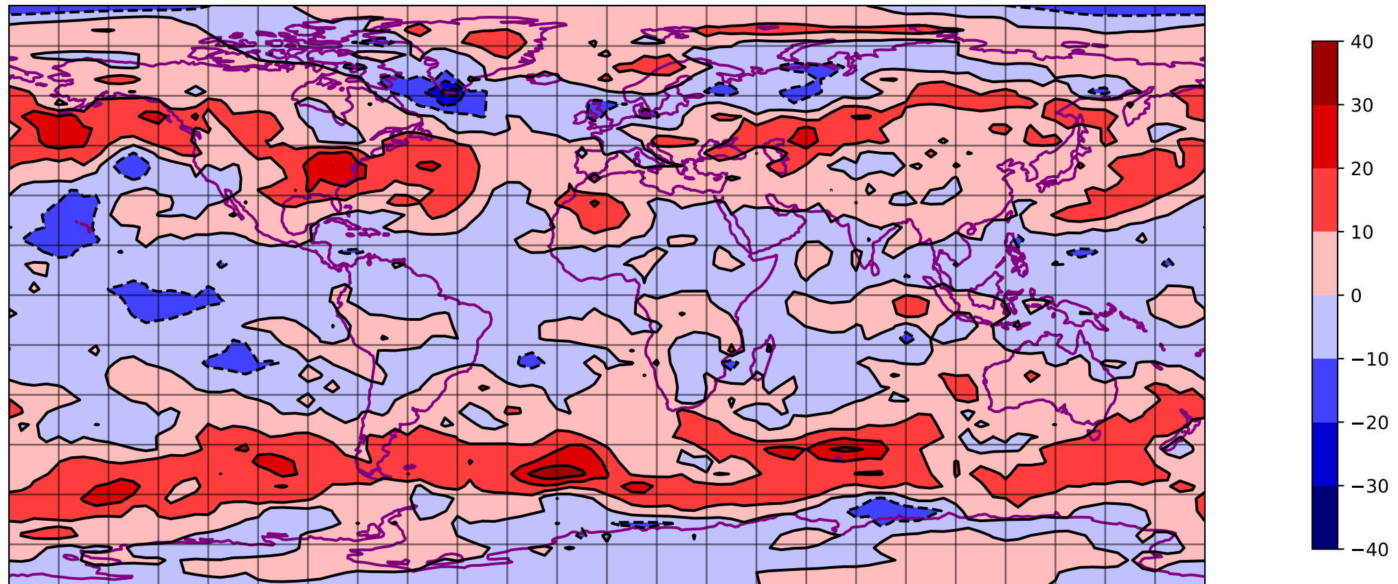
SQG U @ 800 hpa 00 h - T031 ERA5
