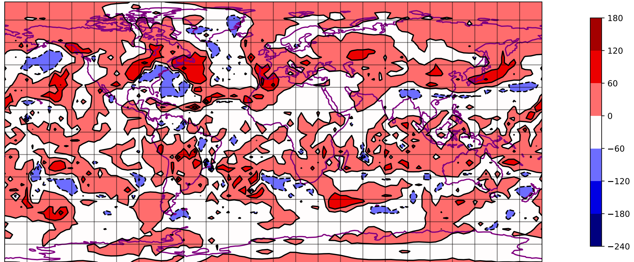
SQG VOR @ 200 hpa 00 h - T031 ERA5
