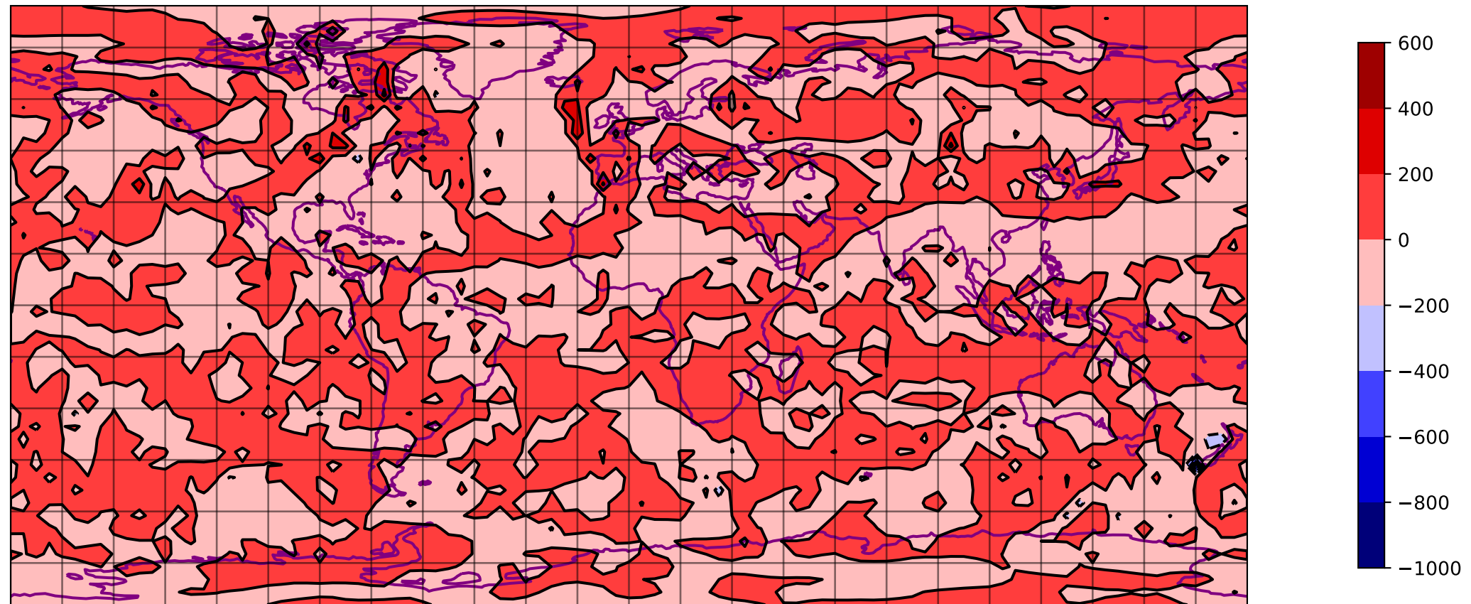
SQG VOR @ 350 hpa 00 h - T031 ERA5
