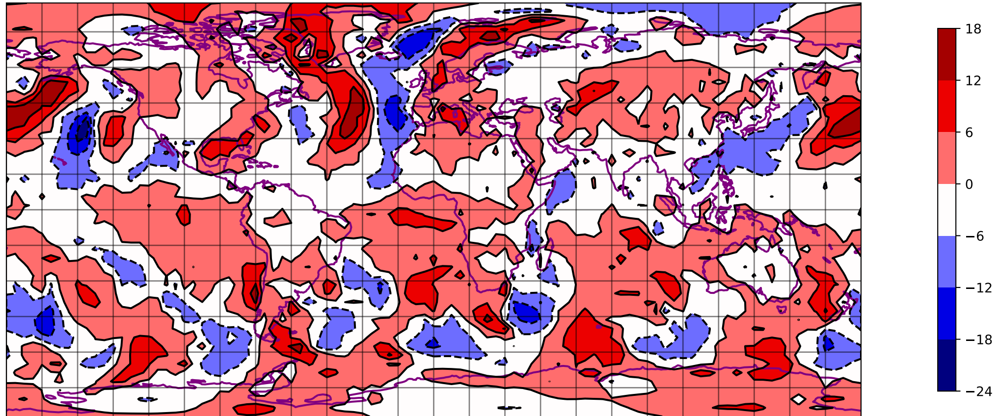
SQG V @ 1000 hpa 00 h - T031 ERA5
