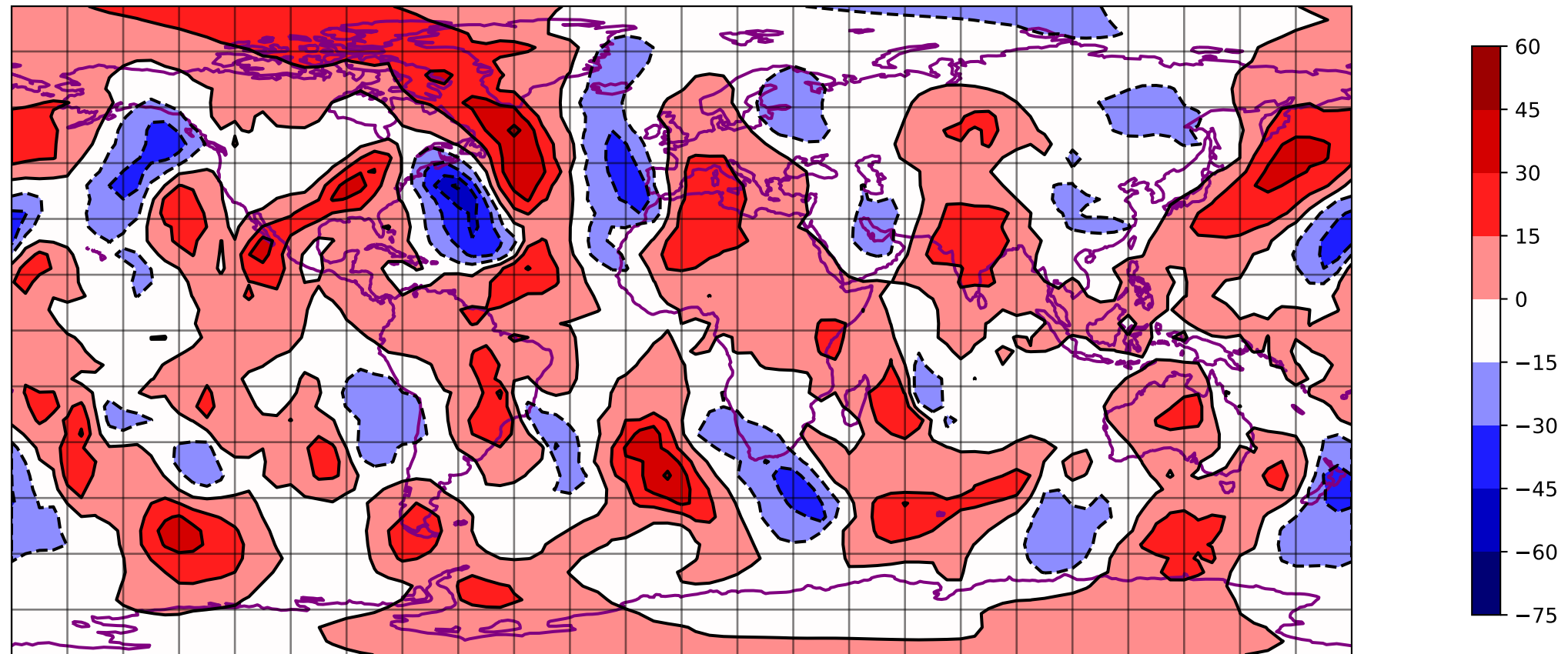
SQG V @ 200 hpa 00 h - T031 ERA5
