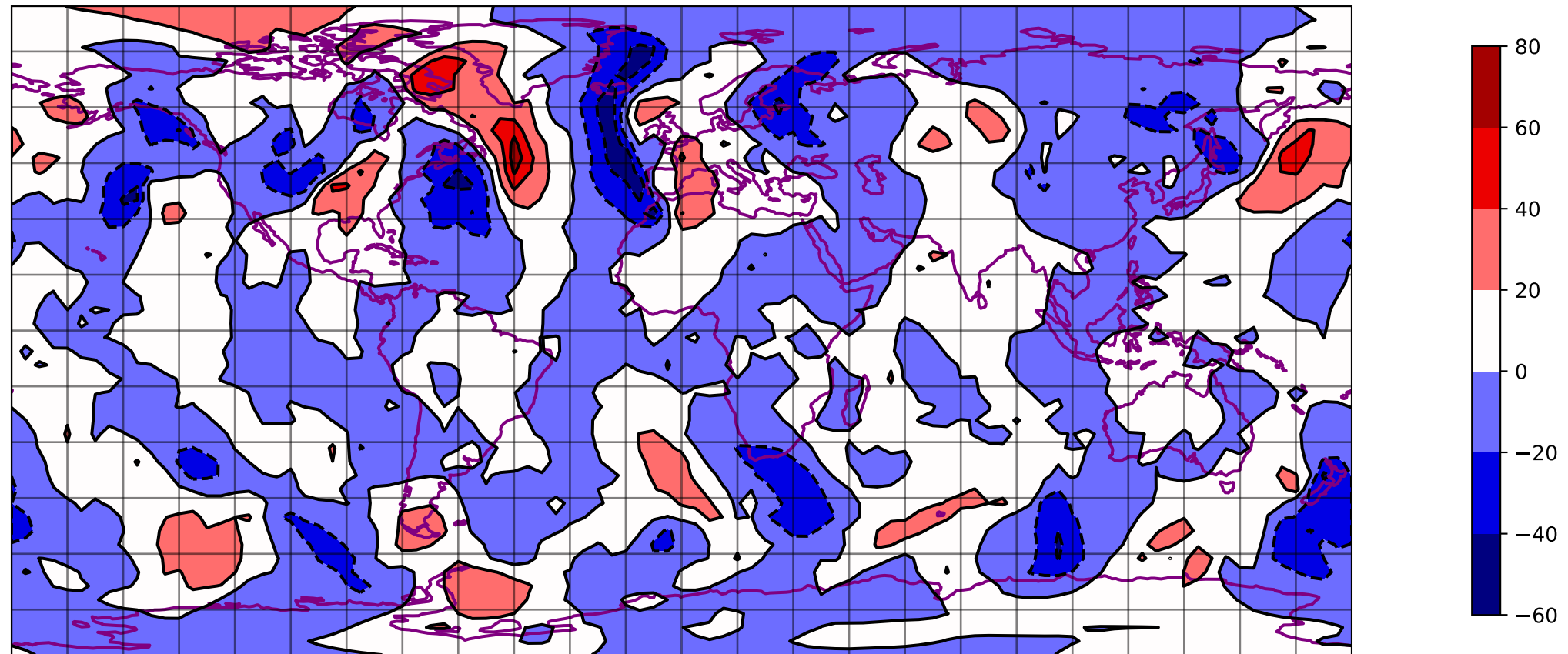
SQG V @ 350 hpa 00 h - T031 ERA5
