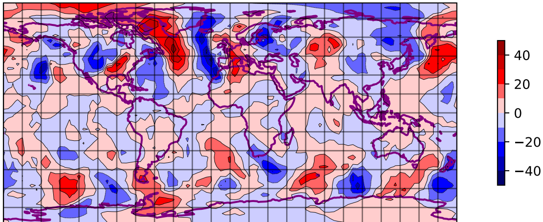
SQG V @ 500 hpa 00 h - T031 ERA5
