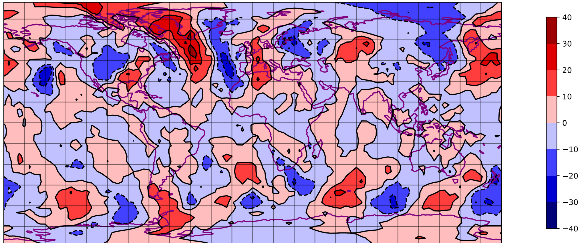
SQG V @ 650 hpa 00 h - T031 ERA5
