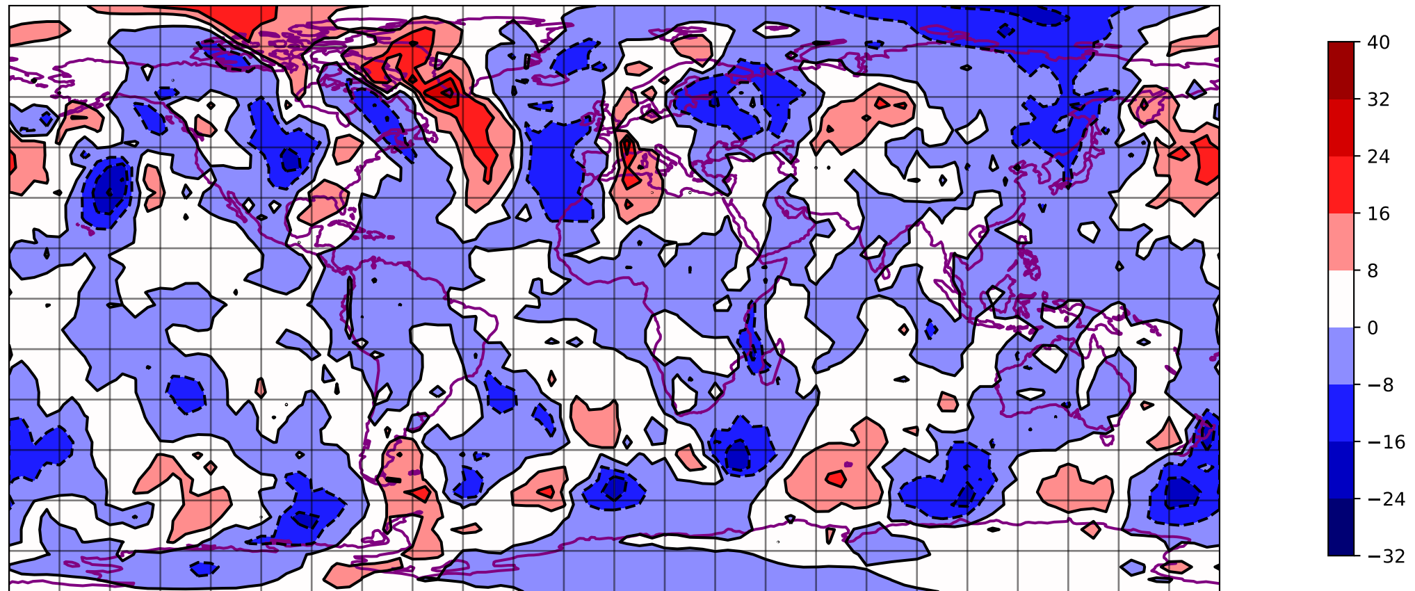
SQG V @ 800 hpa 00 h - T031 ERA5
