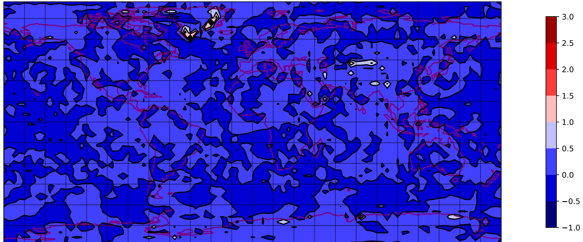
SQG W @ 1000 hpa 00 h - T031 ERA5
