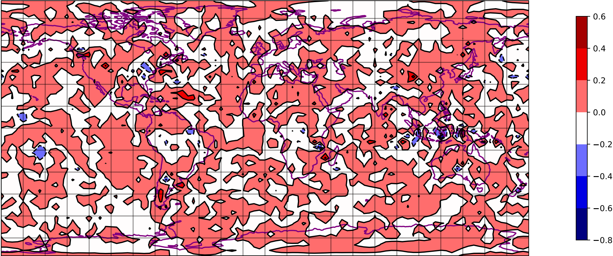
SQG W @ 200 hpa 00 h - T031 ERA5
