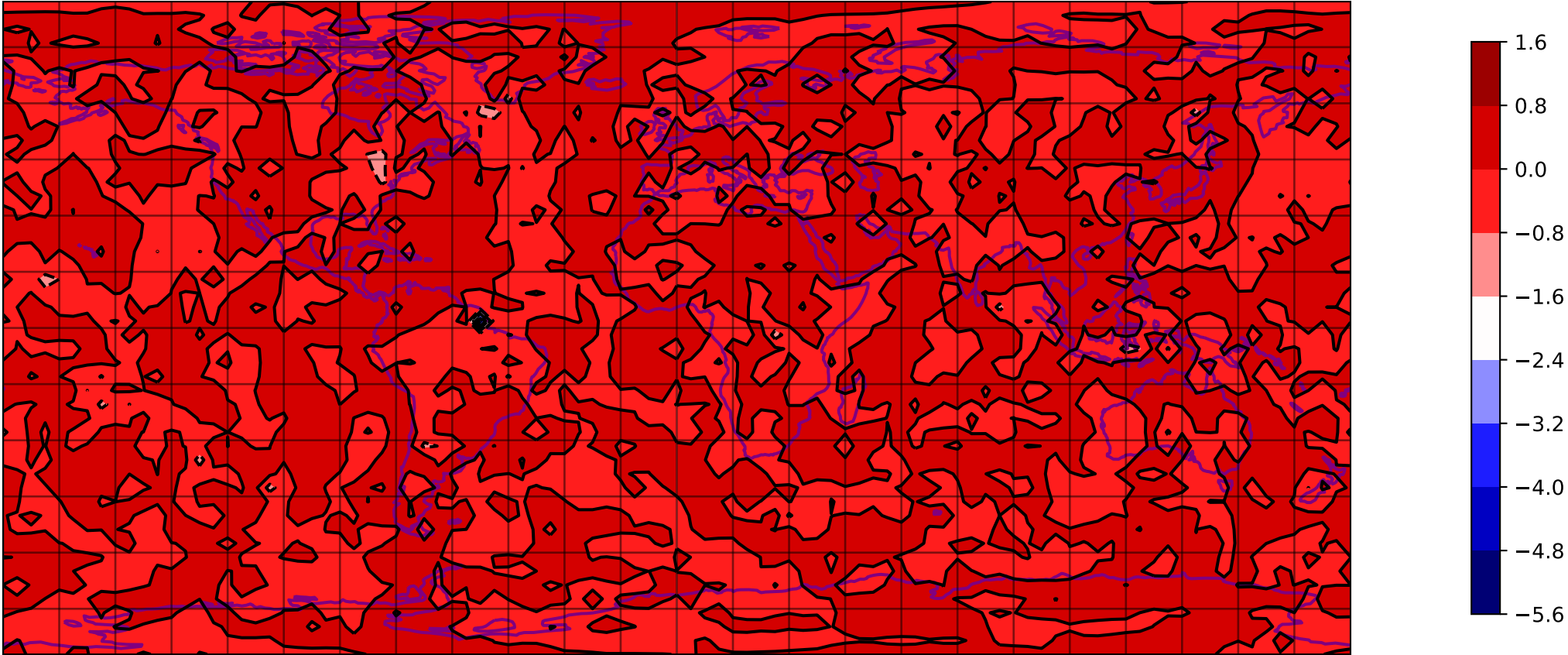
SQG W @ 350 hpa 00 h - T031 ERA5
