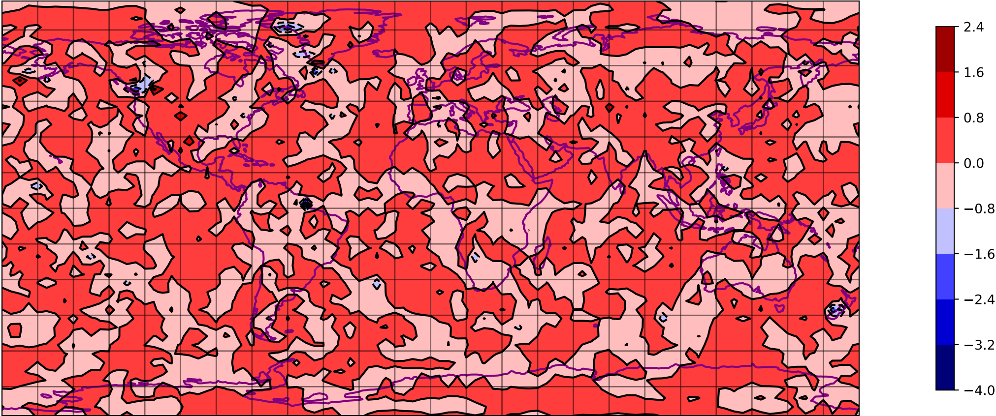
SQG W @ 650 hpa 00 h - T031 ERA5
