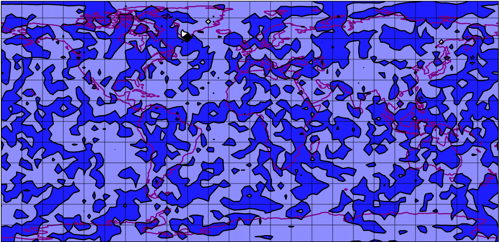
SQG W @ 800 hpa 00 h - T031 ERA5
