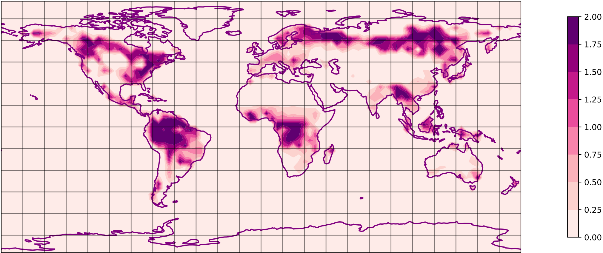
SQG Z0 @ 200 hpa 00 h - T031 ERA5
