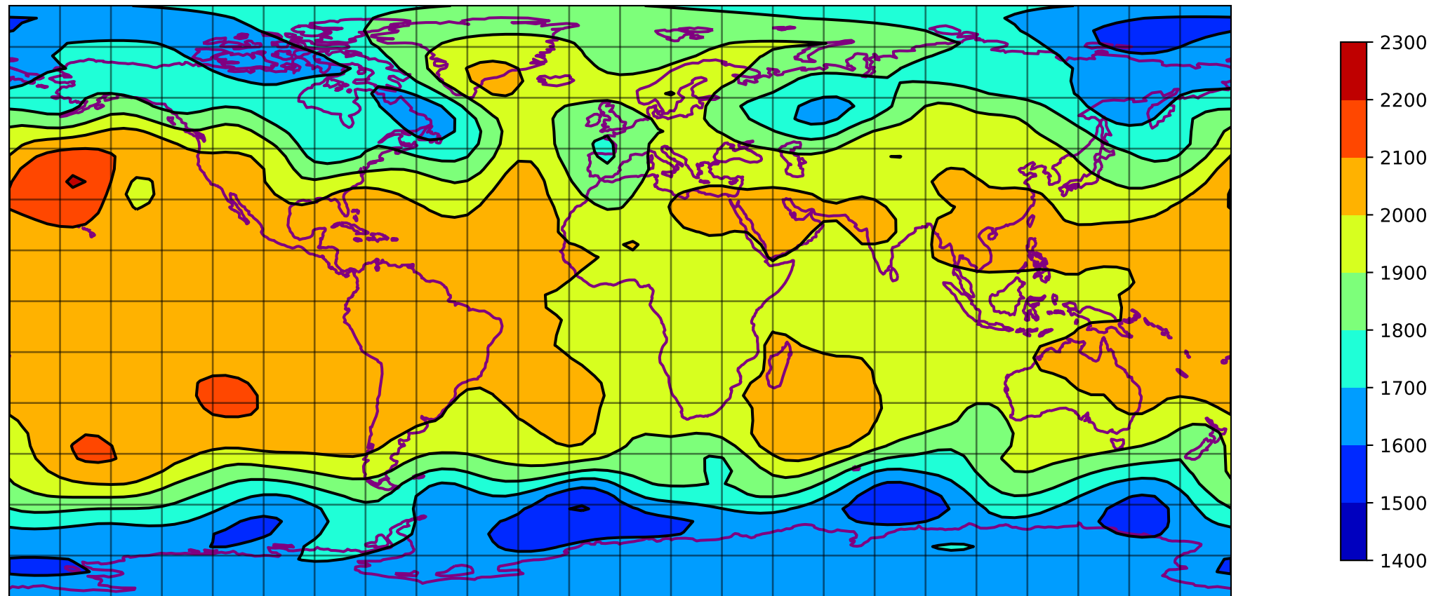
SQG phi 800 hpa 0000h - T031 expid=101
