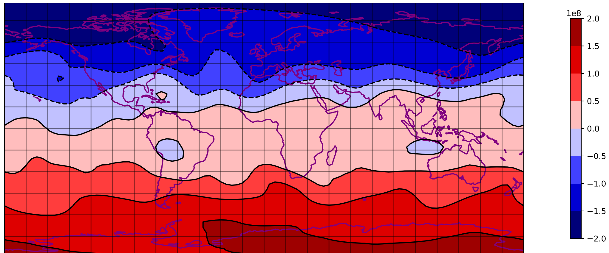
SQG psi 200 hpa 0000h - T031 expid=101
